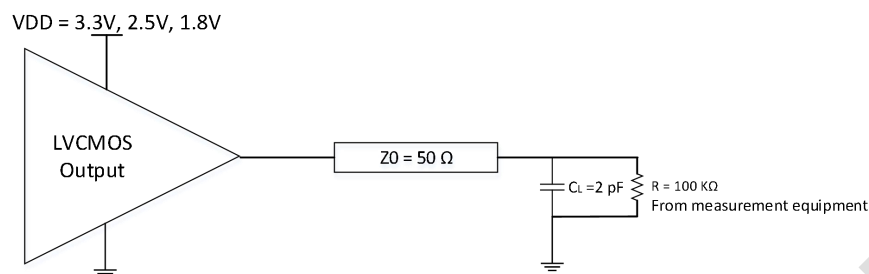
Test Load Circuit
