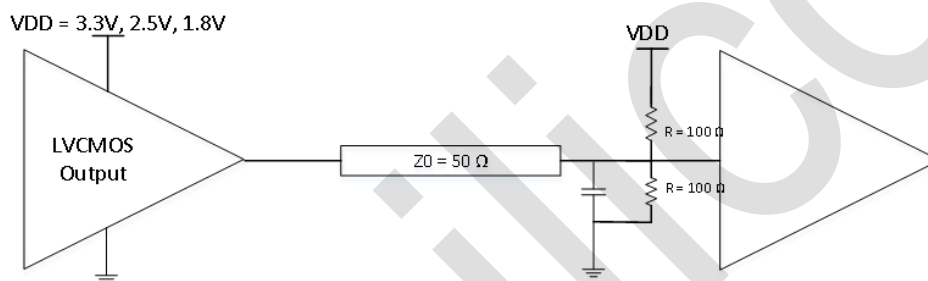
Application Load With 50- \Omega Termination
