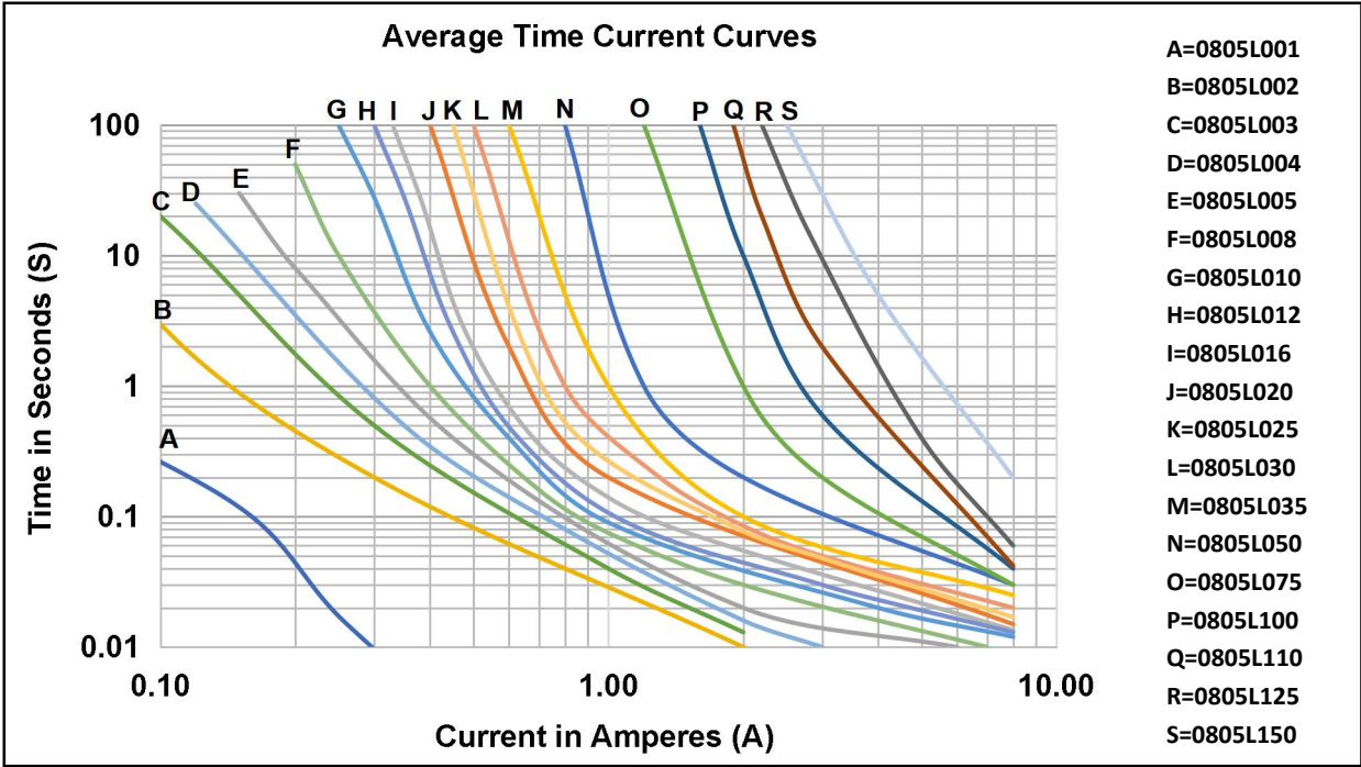
Typical Time-to-Trip at 25°C/25°C跳闸保护时间曲线表
