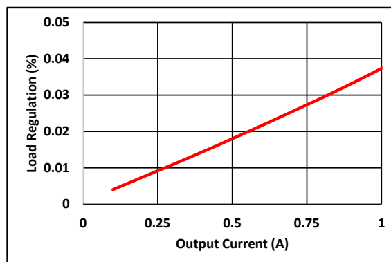
Fig. 4 Load Regulation
