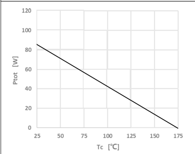
Figure 4. Power Dissipation
