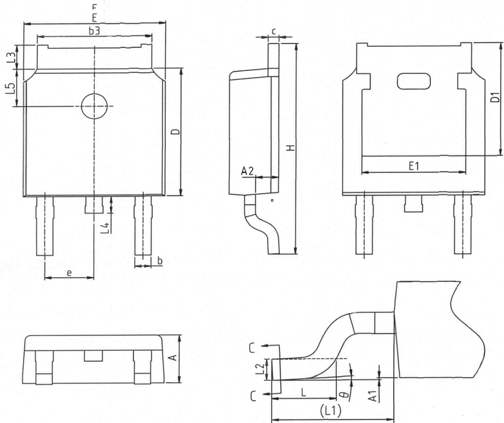
COMMON DIMENSIONS
