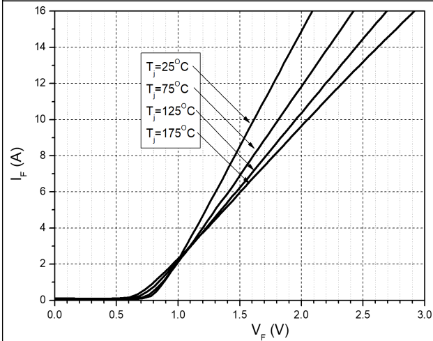
Figure 1. Forward Characteristics
