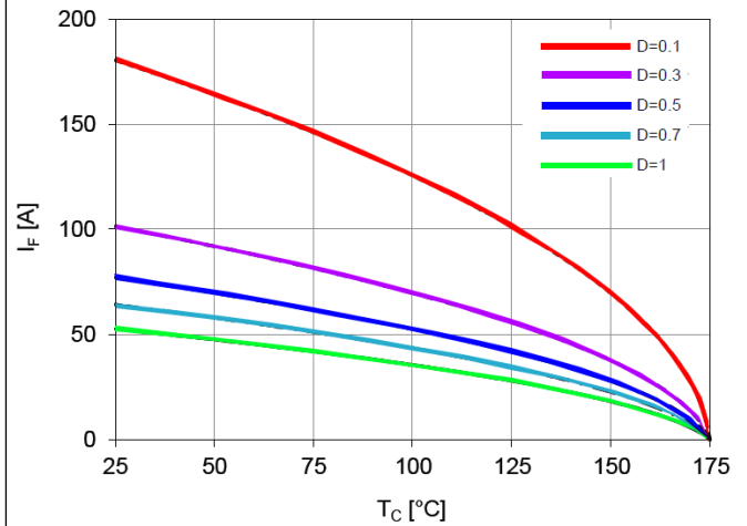
Figure 2. Current Derating
