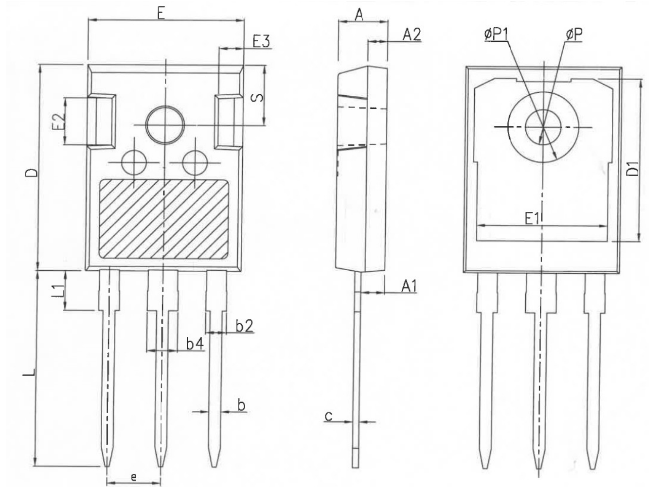
COMMON DIMENSIONS
