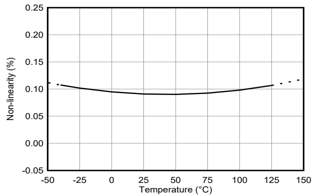
Figure 6-3. Non-Linearity vs Temperature
