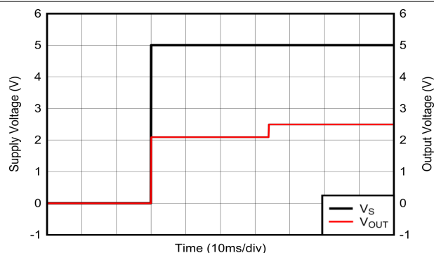
Figure 6-12. Startup Transient Response
