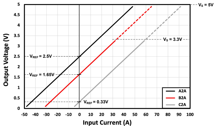
Figure 8-4. Output Voltage Relationship to Input Current for TMCS1126x2A
