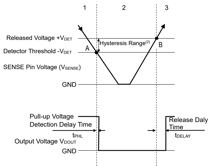
Diagram for R3121xxxE with External Capacitor
