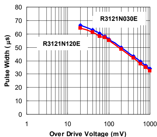
R3121NxxxE Pulse Width vs. Over Drive Voltage
