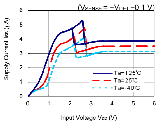
R3121NxxxE ( V_{\text{SENSE}} = -V_{\text{DET}} - 0.1 \text{ V} )
