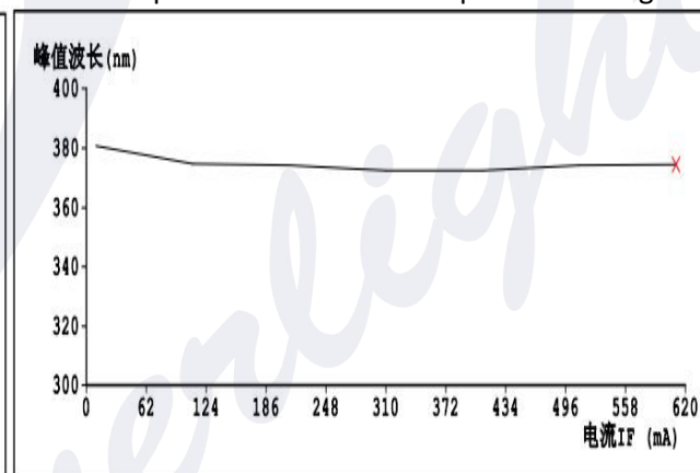
Spectral wavelength
