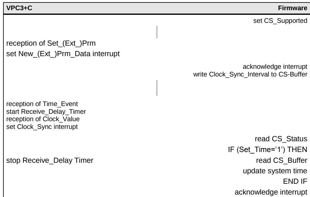
Figure 7-24: communication scheme
