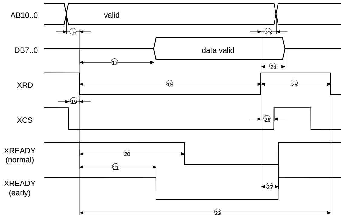
Figure 10-12: Asynchronous Intel Mode, READ ( XWR = 1 )
