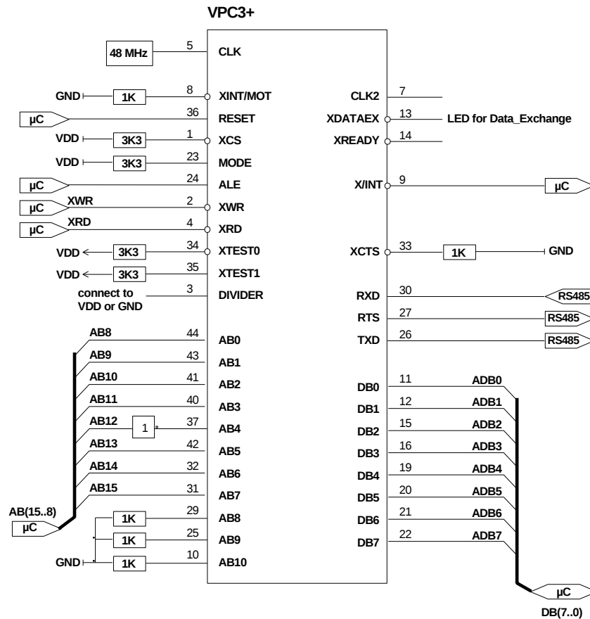
Figure 8-6: 80C32 Application in 2K Byte mode
