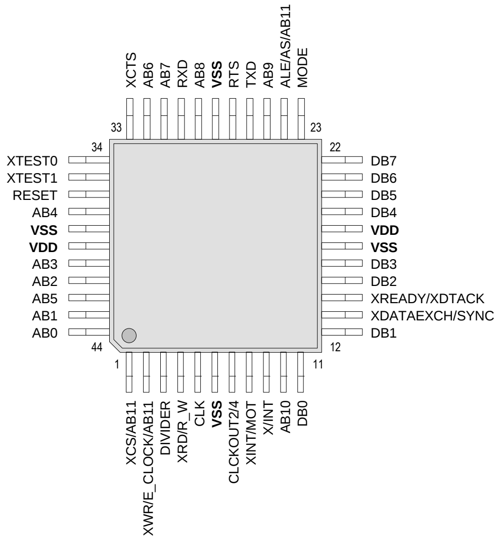
Figure 3-3: VPC3+C Pinout
