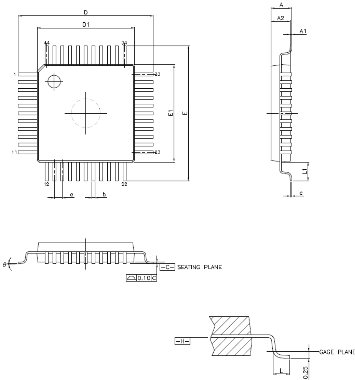
Figure 10-21: Package Drawing
