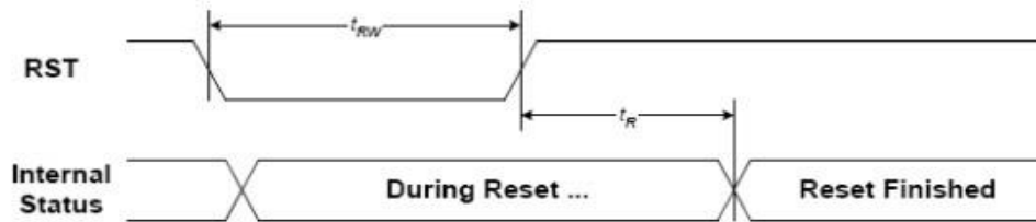
FIGURE 15: Reset Characteristics
