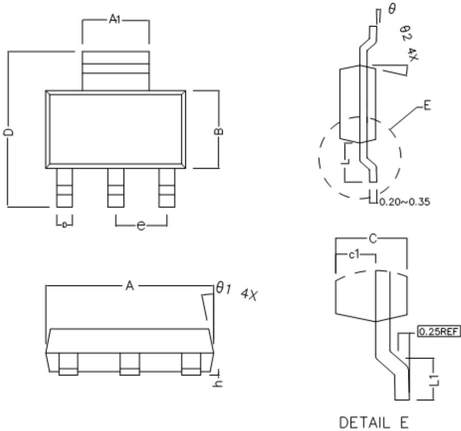
SOT-223 Package Outline Dimensions (Units: mm)
