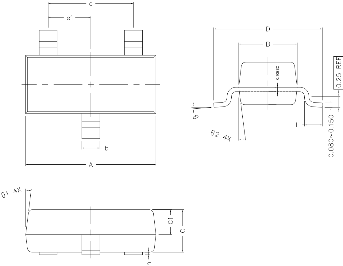
SOT-23 Package Outline Dimensions (Units: mm)
