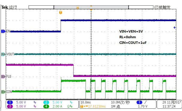
Short Circuit Response
