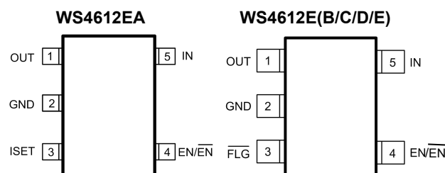
Pin configuration (Top view)
