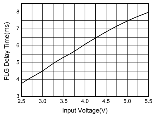
FLAG delay time vs. Input Voltage
