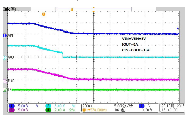
Shutdown from Power OFF
