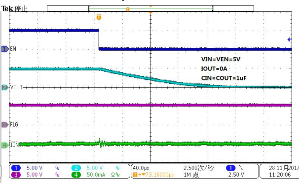
Shutdown from Enable OFF
