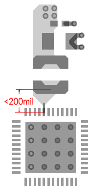
Figure 20. REG_OUT Pin PCB Design
