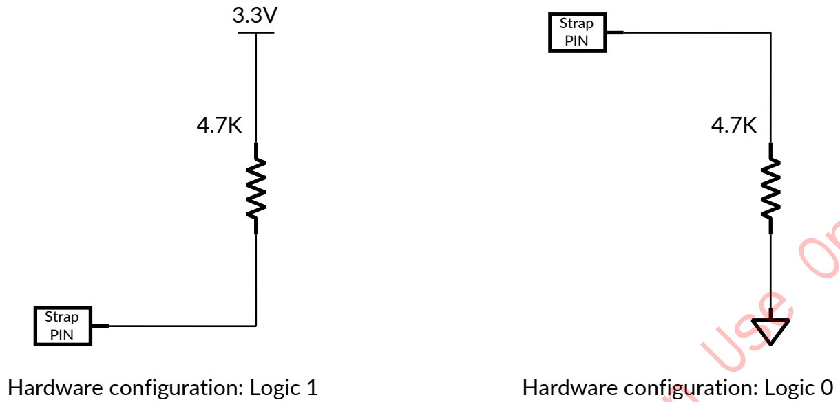
Figure 10. Hardware Configuration Reference Design
