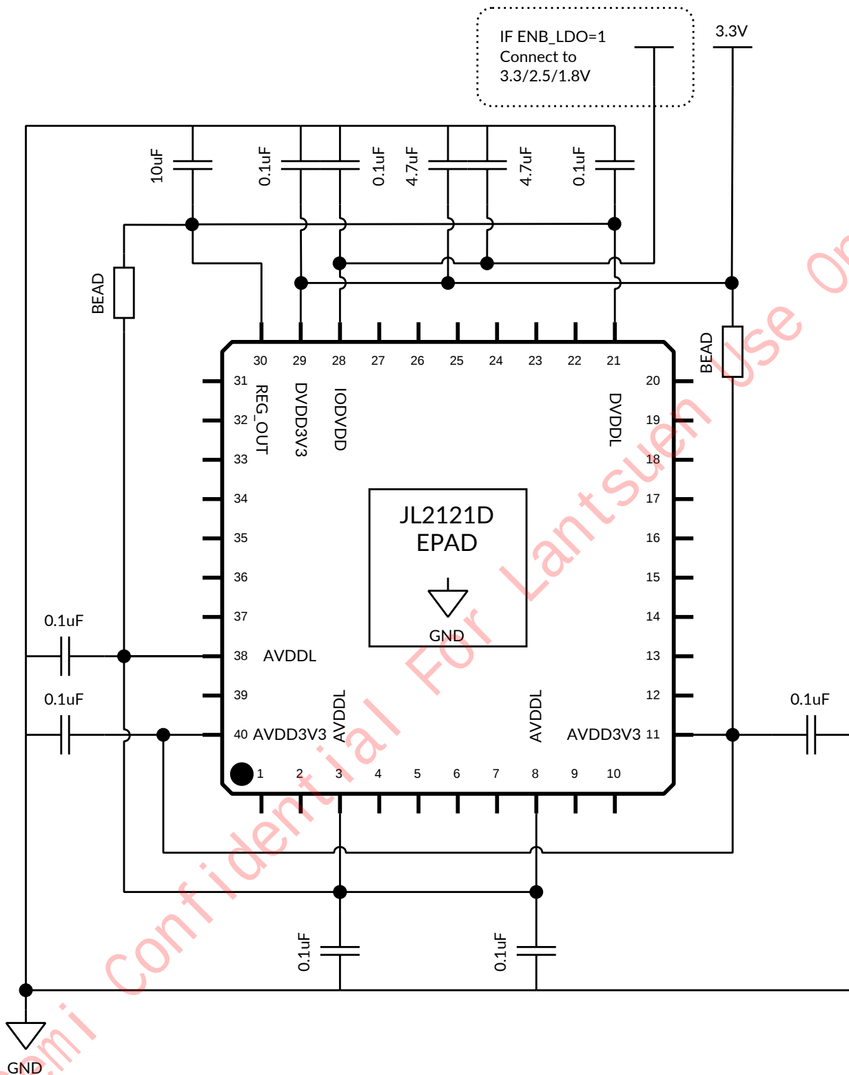
Figure 18. JL2121D Power Interface Reference Design
