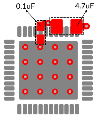
Figure 21. Power Decouple Design
