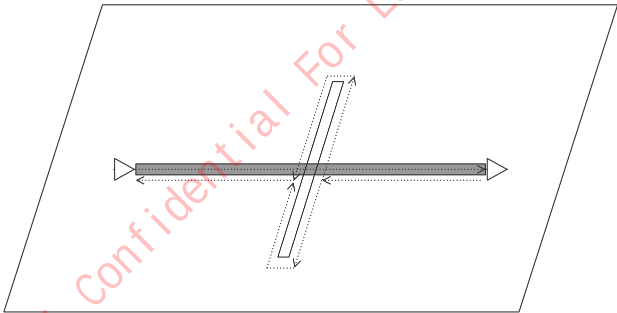
Figure 23. Slot in Reference Plane
