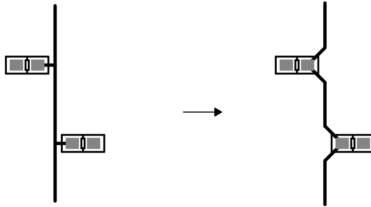
Figure 24. Avoid Stub Traces by Daisy Chain Routing
