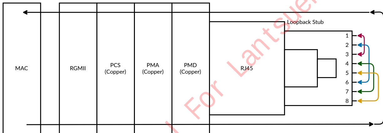
Figure 13. External Loopback Path
