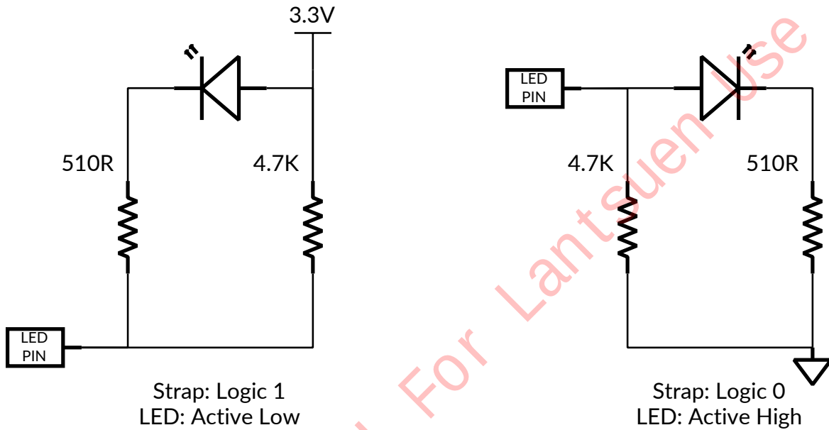
Figure 16. LED Duplex with Strap Reference Design
