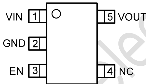
Top View SOT23-5
