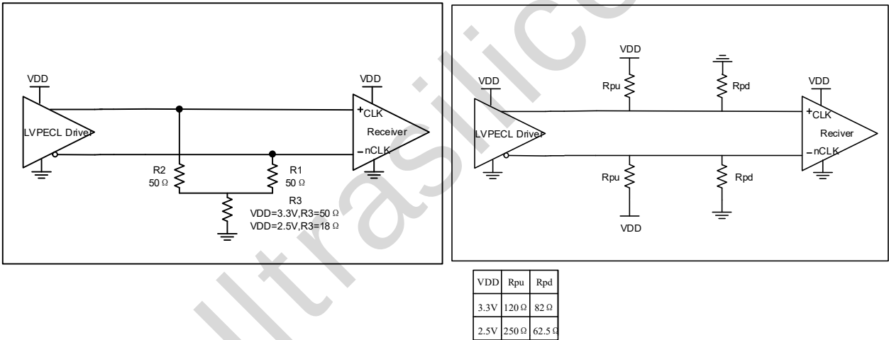
Figure6.LVPECL Driver(DC)
