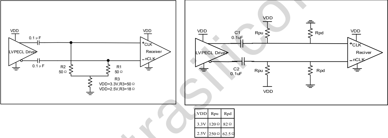
Figure5.LVPECL Driver(AC)
