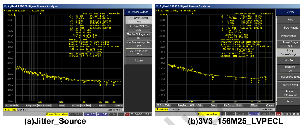
Figure 1 .RMS_Jitter_3V3=√(92 2 -44 2 )=81fs
