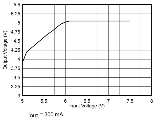
图 8-32. Drop-Out Response
