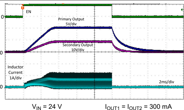
图 8-7. Full Load Start-Up from EN
