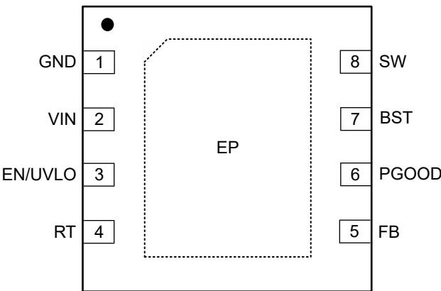
图 5-2. 8-Pin WSON NGU Package (Top View)
