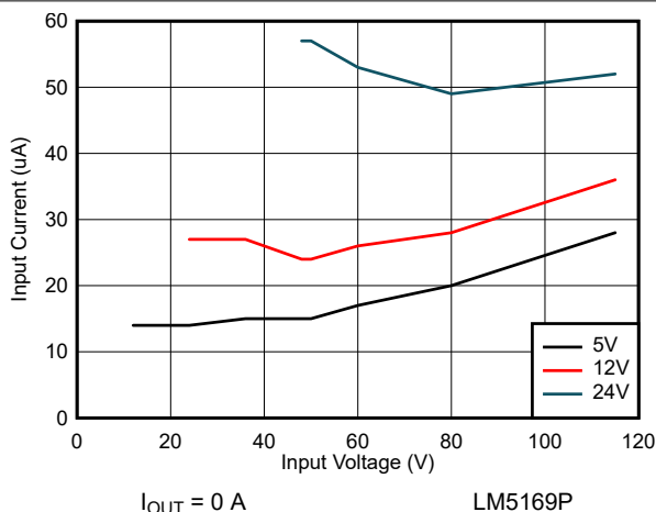
图 8-30. No-Load Input Supply Current
