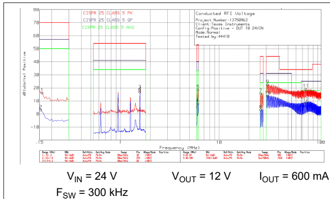
图 8-37. LM5169PDDAR Conducted EMI (Positive Rail)
