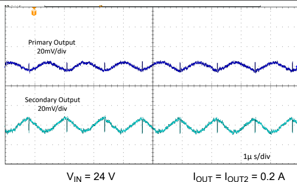
图 8-13. Typical Output Ripple
