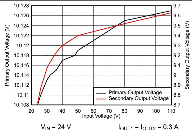
图 8-5. Line Regulation
