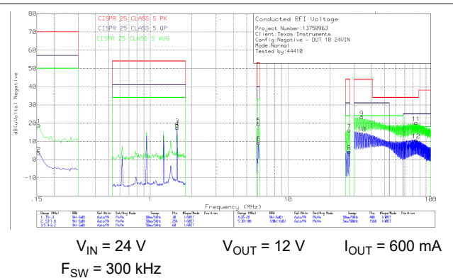
图 8-38. LM5169PDDAR Conducted EMI (Negative Rail)
