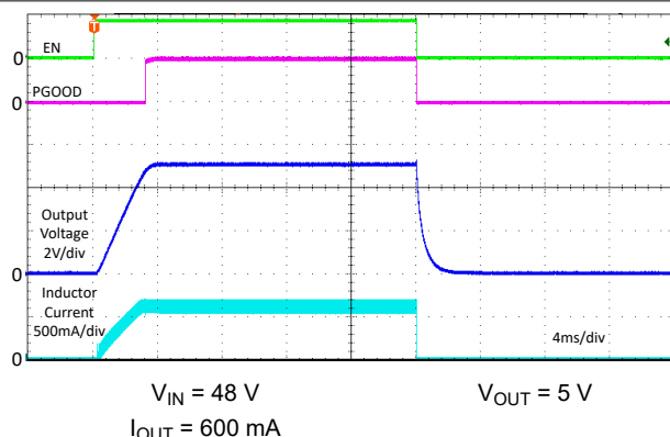
图 8-29. Typical Start-up Waveforms
