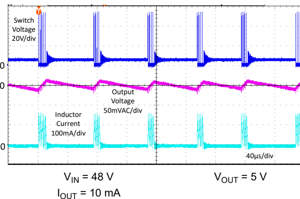
图 8-28. Typical Switching Waveforms
