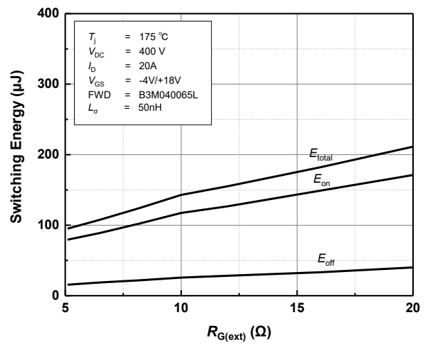
Figure 20 Clamped Inductive Switching Energy vs. External Gate Resistance at T_j = 175^\circ\text{C}
