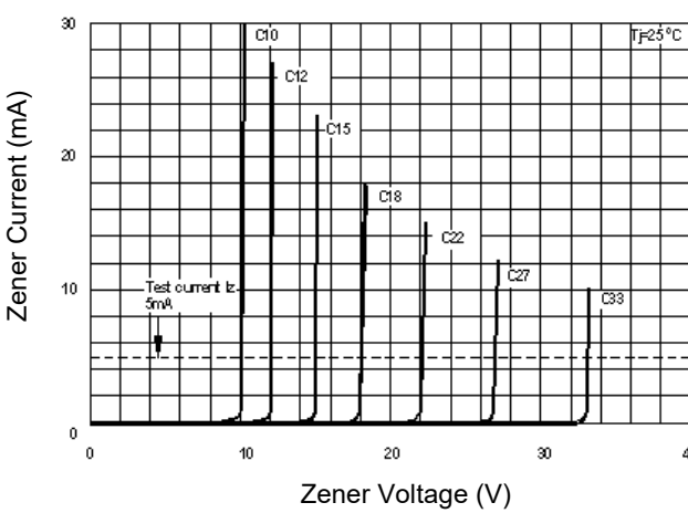
Fig.2 Zener Characteristics Curve
