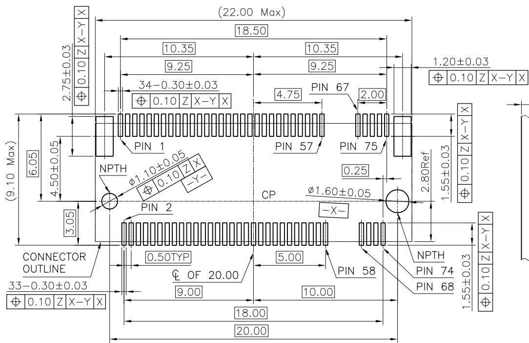
RECOMMENDED PCB LAYOUT(TOP VIEW) DEFAULT TOLERANCE ±0.05MM
