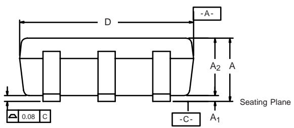
5-LEAD TSOP
