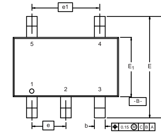
5-LEAD TSOP
