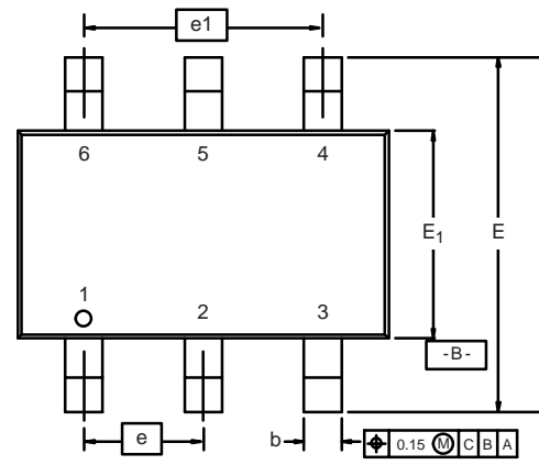
6-LEAD TSOP
