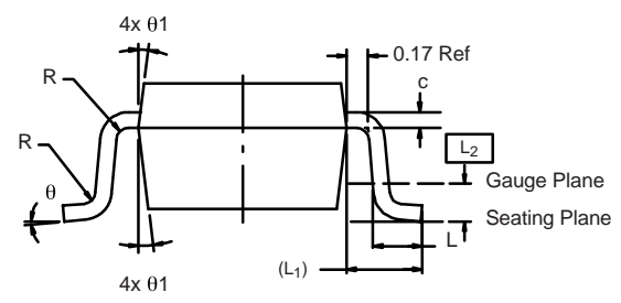
6-LEAD TSOP
