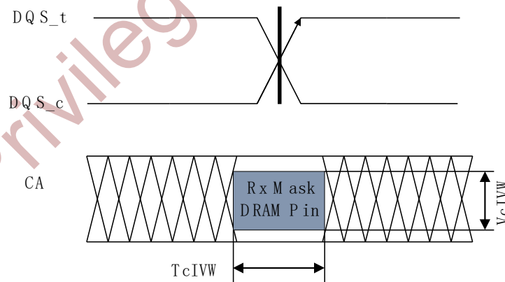
Figure 8-23 CA Timings at the DRAM Pins
