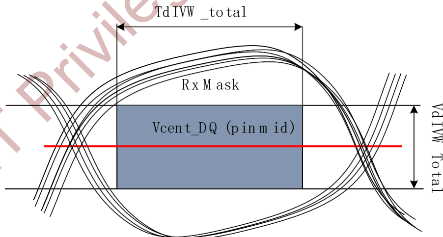
Figure 8-28 DQ Receiver(Rx) Mask
