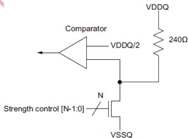
Figure 5-19 Pull-down Calibration
