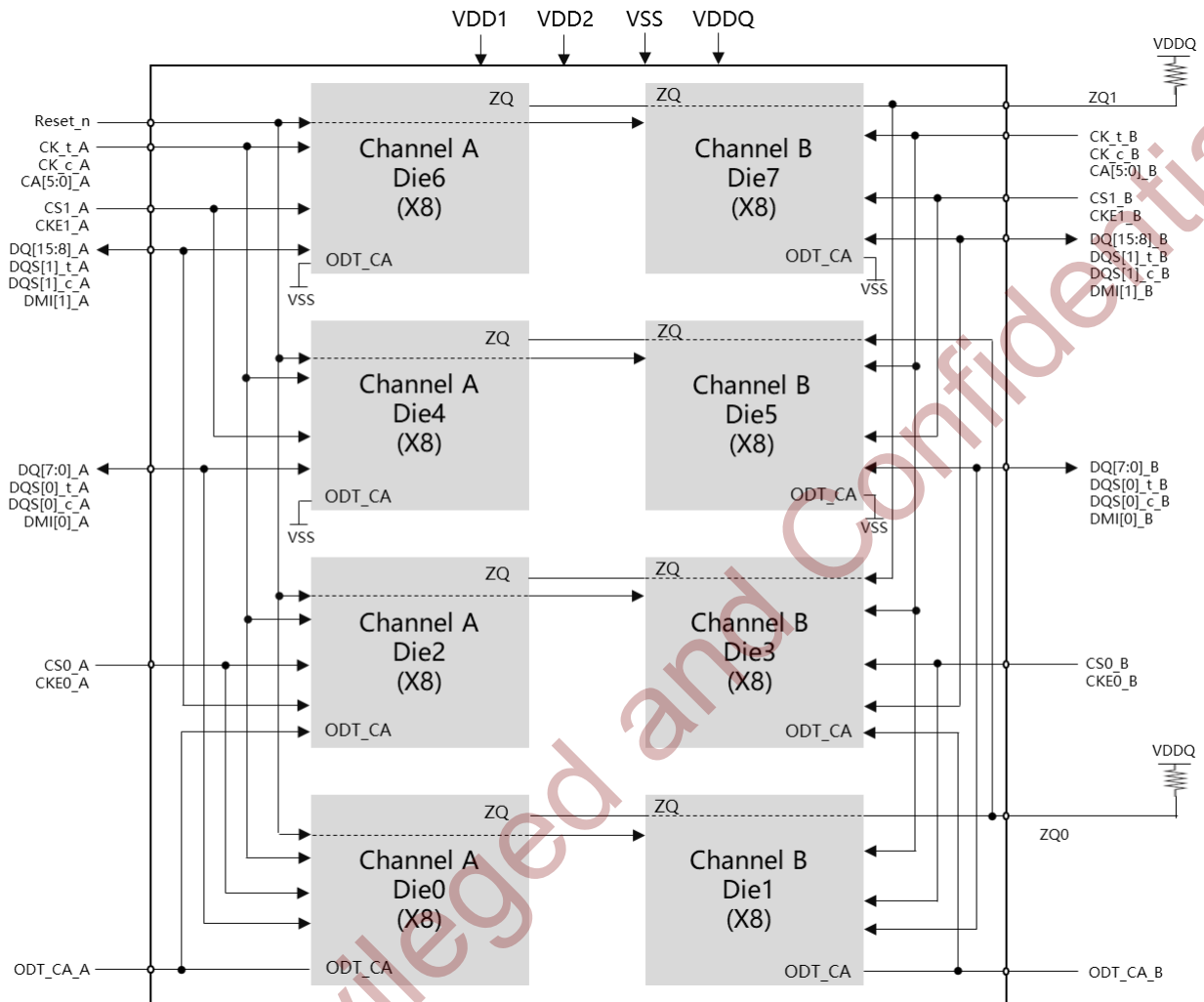
Figure 2-3 Octo-Die, Dual-Channel, Dual-Rank Package Block Diagram (8GB x32 I/O)
