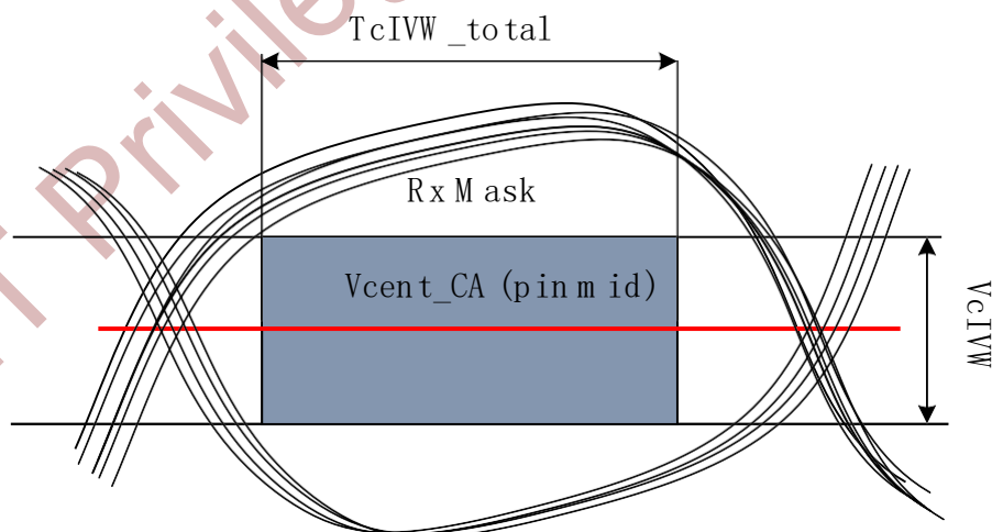
Figure 8-21 CA Receiver(Rx) Mask
