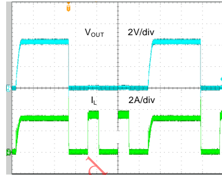
Short Circuit Protection ( V_{IN}=5.0V , V_{OUT}=4.2V , I_{OUT}=3 - Short)
