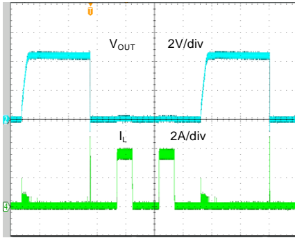
Short Circuit Protection ( V_{IN}=5.0V , V_{OUT}=4.2V , I_{OUT}=0 - Short)
