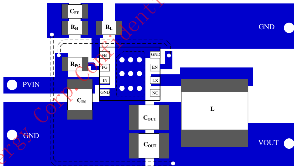
Figure4. PCB Layout Suggestion
