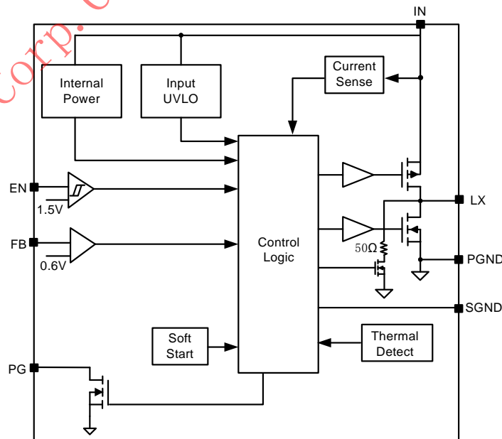
Figure3. Block Diagram
