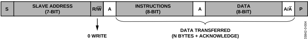
Figure 24. I 2 C—Master Writing Data to Slave
