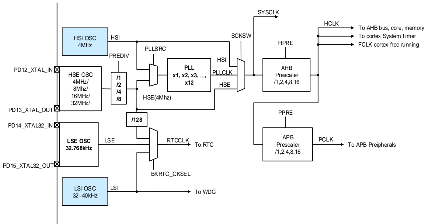
Figure 4.3-1: Clock Tree
