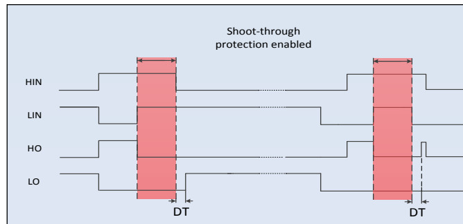
Figure 4.15-4.15-4: Shoot-through Prevention
