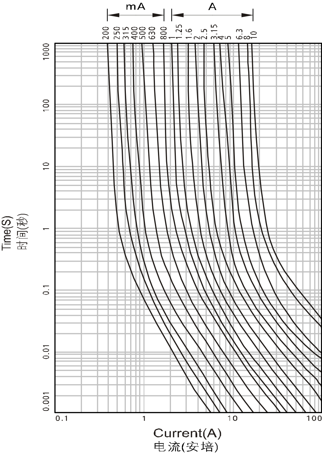
Time-Current Characteristics 电流-时间曲线图
