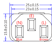
ME-302 (IEC 60320, C13, 13A 125V~) (Dimensions of Connector Face)
