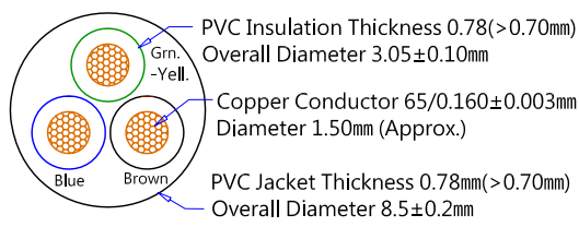
SJT 16AWGx3C (Wire Cross-Section)
