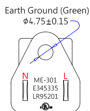
ME-301 (NEMA 5-15P) (Dimensions of Plug Face)
