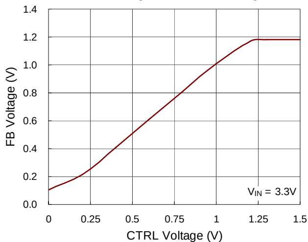
FB Voltage vs. CTRL Voltage
