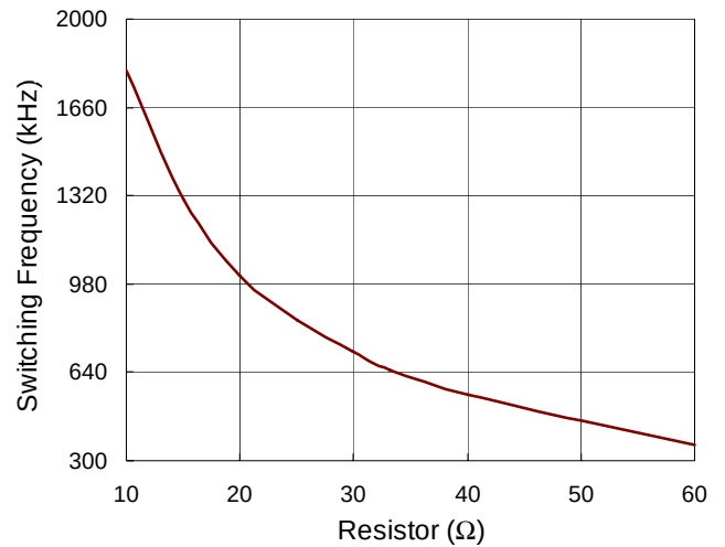
Switching Frequency vs. Resistor
