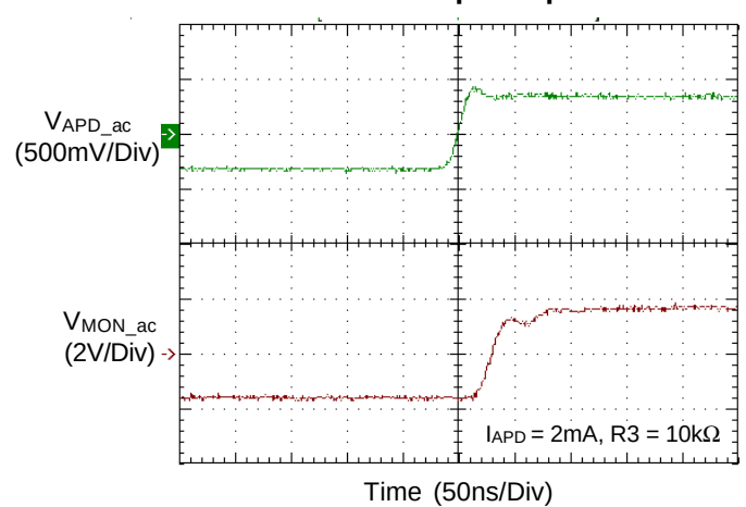
Monitor Step Response
