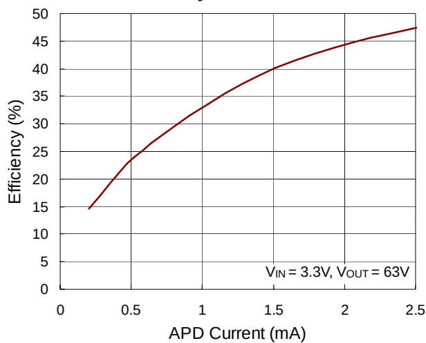
Efficiency vs. APD Current
