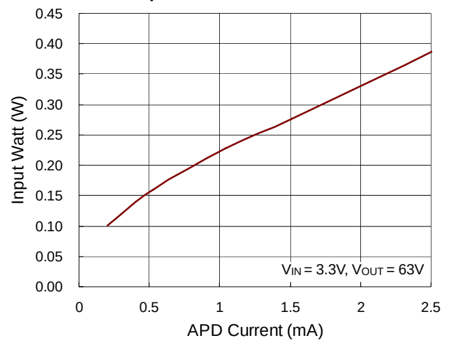
Input Watt vs. APD Current
