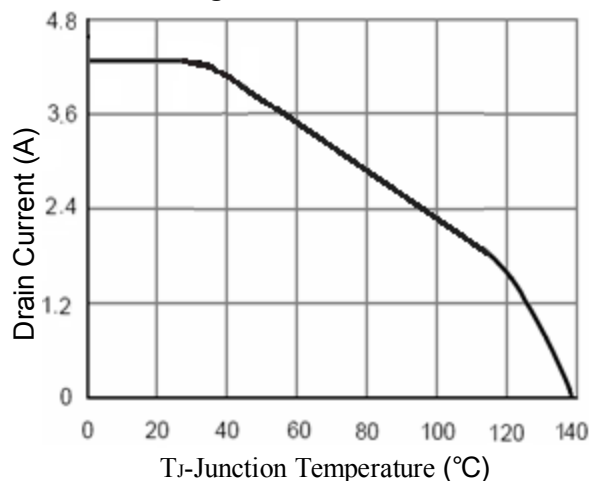
Figure2. Drain Current
