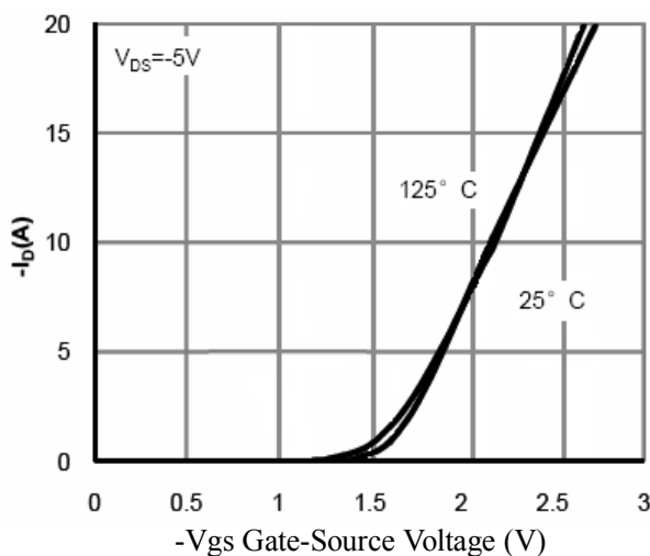
Figure4. Transfer Characteristics
