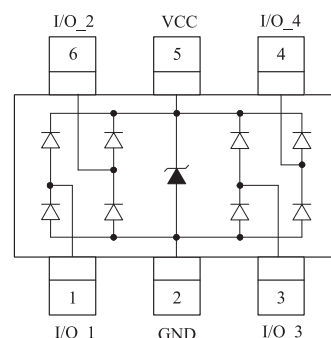
SOT23-6L (Top View)
