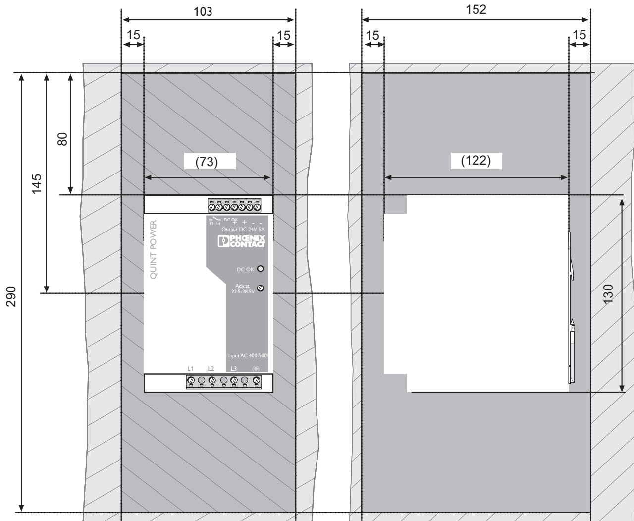
Dimensioned drawing
