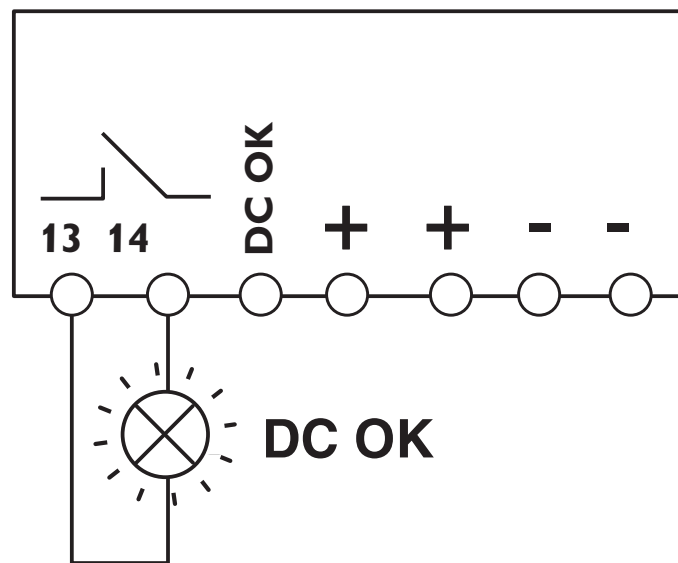
Circuit diagram
