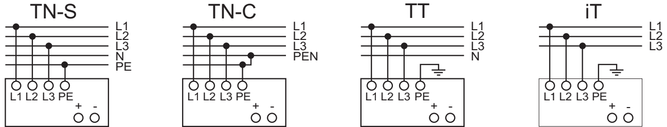
Connection diagram
