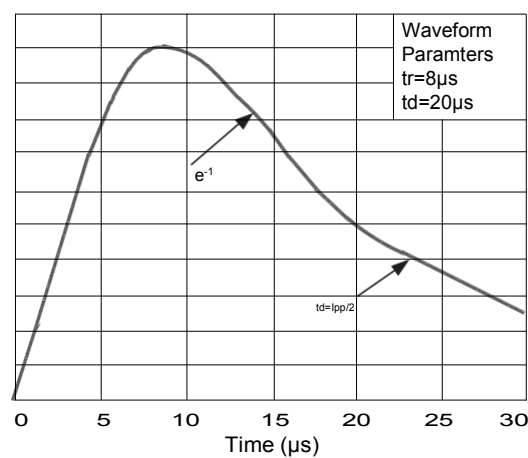
Figure3: Pulse Waveform
