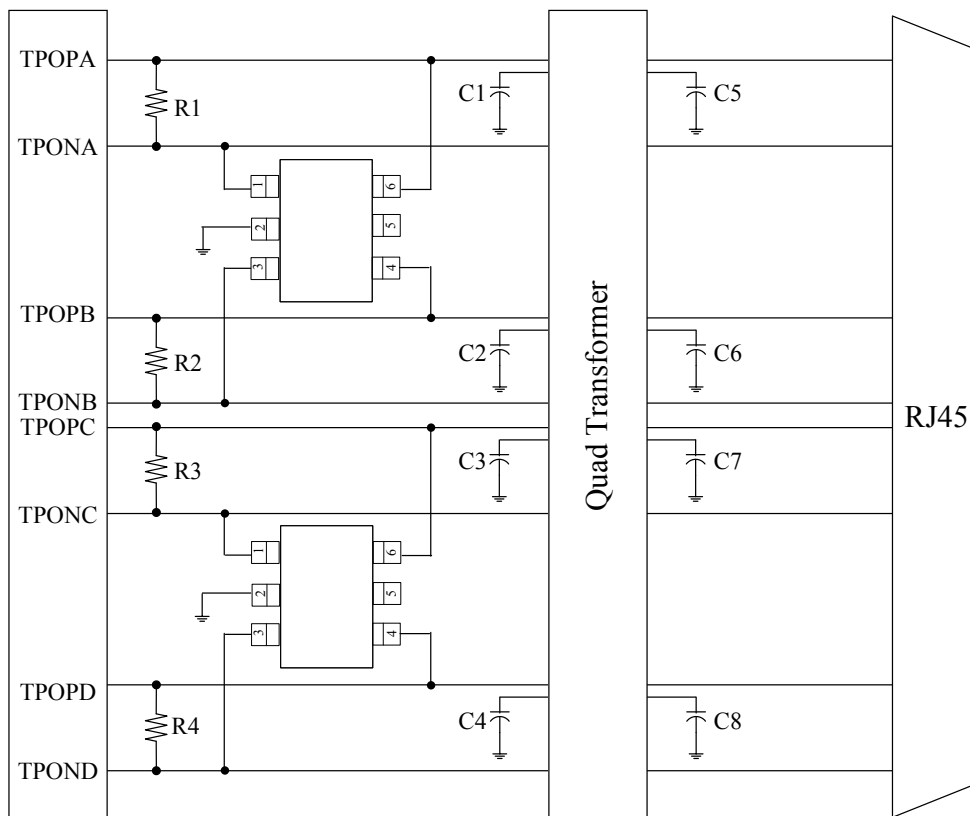
Schematic Diagram for Gigabit Ethernet ESD/Surge Protection using TS3314VL
