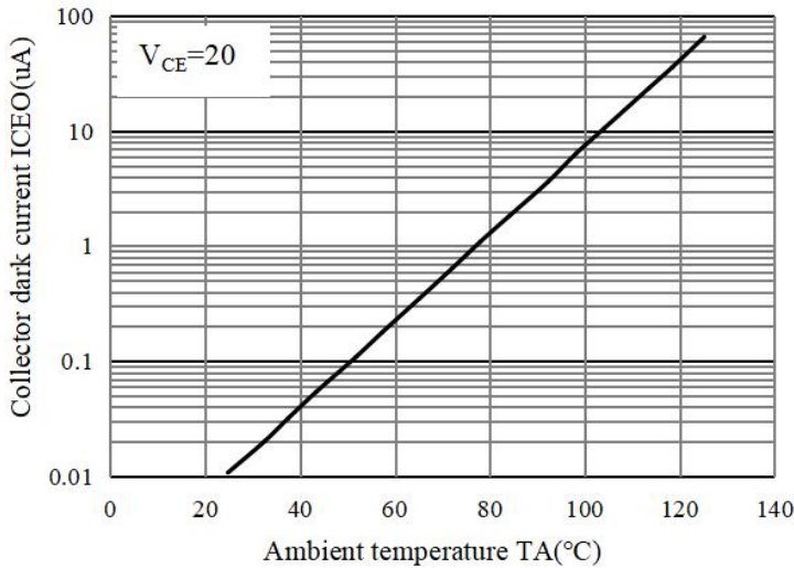
Fig.9 Collector Dark Current vs. Ambient Temperature
