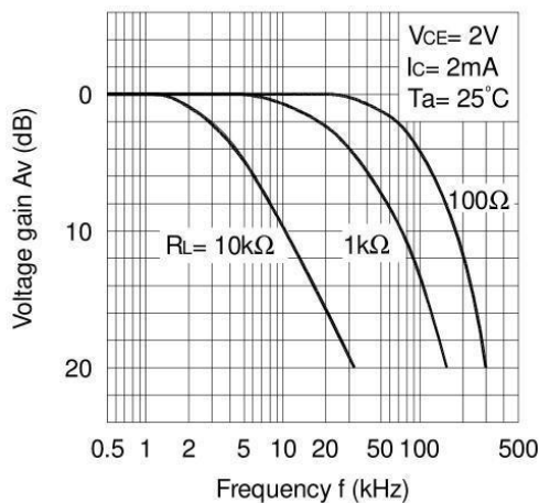
Fig.11 Frequency Response
