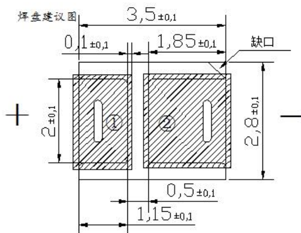
焊点结构 Pad Configuration:
