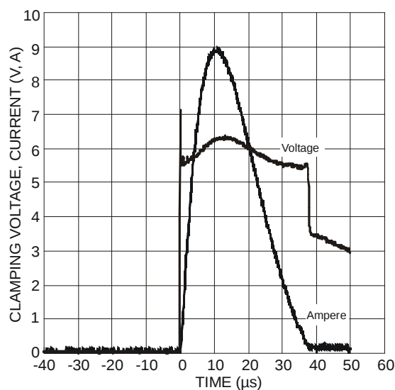
Figure 6 Waveform of Clamping Voltage, Current vs. Time (8/20μs, V CC to V SS )
