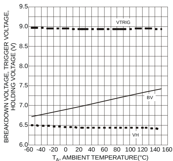
Figure 2 Breakdown Voltage, Trigger Voltage, Holding Voltage vs. Ambient Temperature
