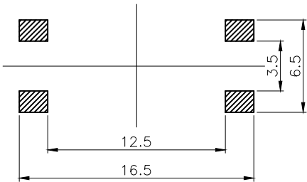
PCB WELDING DRAWING
