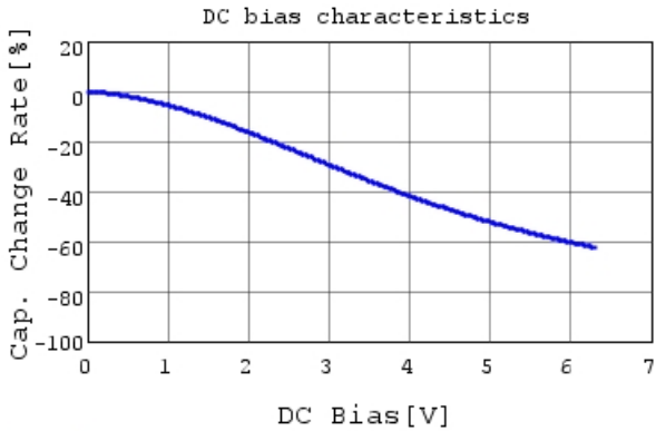
GRM219R60J106ME19 C-DC bias capchange, 25.0c
