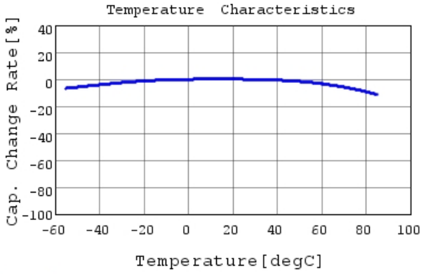
GRM219R60J106ME19 C-Temp. capchange, DC0.0V,
