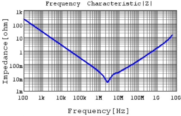
GRM219R60J106ME19 |Z| DCOV, 25degC
