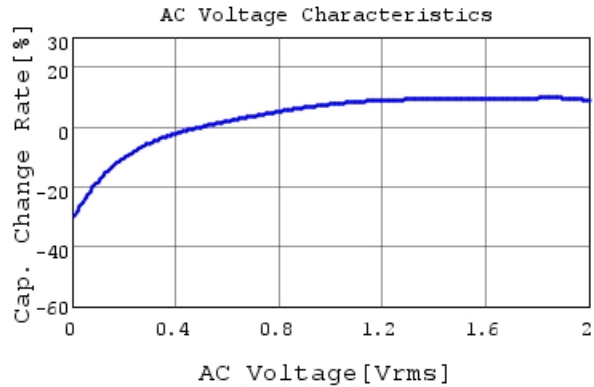
GRM219R60J106ME19 C-AC Voltage capchange, DC
