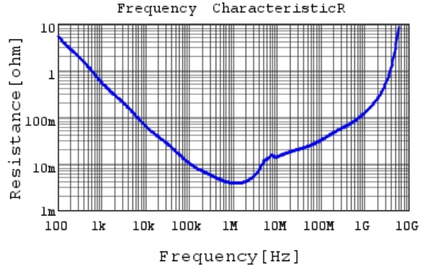
GRM219R60J106ME19 R DCOV, 25degC
