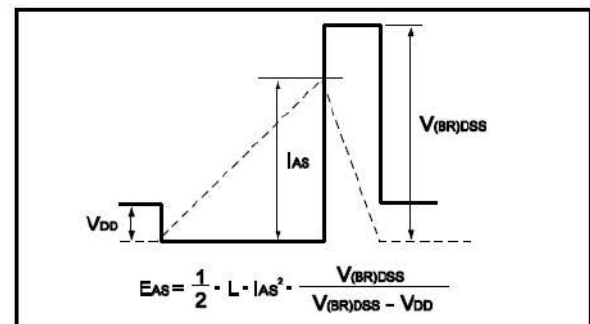
Fig.12 Avalanche Waveform
