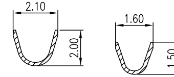
SEC A-A SEC B-B FOR WIRE SIZE AWG#26~30
