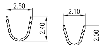
SEC A-A SEC B-B FOR WIRE SIZE AWG#20~24
