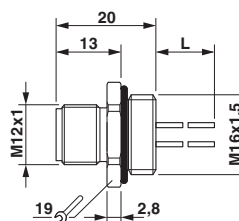
Dimensional drawing
