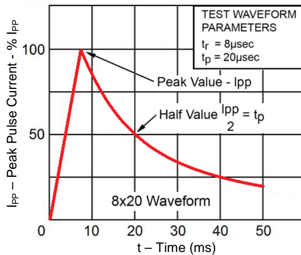
FIGURE 2 8/20 \mu s CURRENT IMPULSE WAVEFORM
