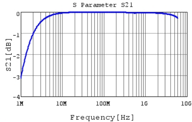
GCM1885C2A152JA16 S21 DCOV, 25degC
