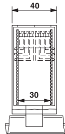
Dimensional drawing
