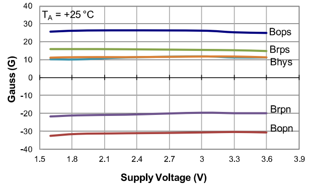
Switch Points vs Supply Voltage
