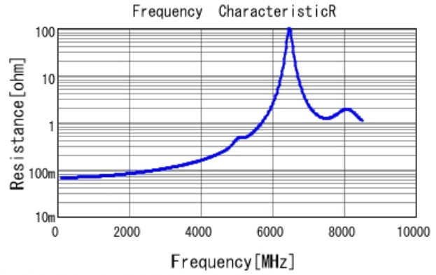
■ GQM1875G2E8R0BB12 R DCOV, 25degC
