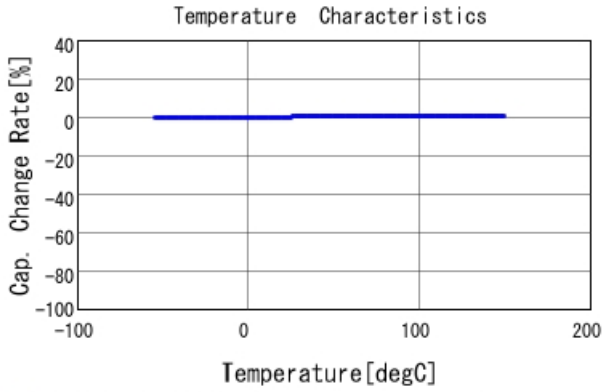
■ GQM1875G2E8R0BB12 C-Temp. capchange, DCOV, AC1Vrms
