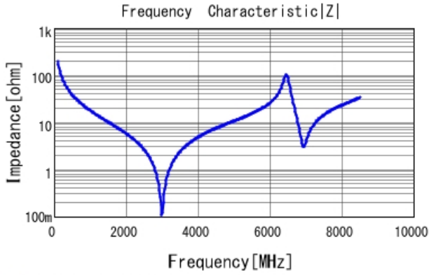
■ GQM1875G2E8R0BB12 |Z| DCOV, 25degC
