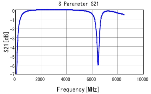
■ GQM1875G2E8R0BB12 S21 DCOV, 25degC
