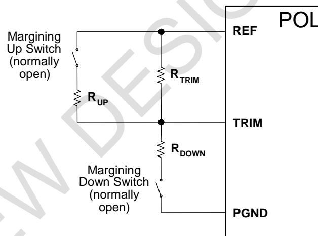
Figure 19. Alternative Margining Configuration
