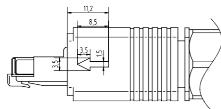
Connector Marking
