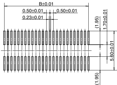
Recommended metal mask pattern Metal mask thickness: Here, 120 µm (Opening area ratio: 78%)
