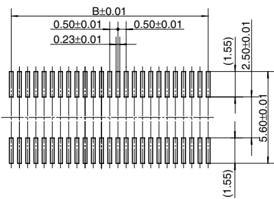
Recommended metal mask pattern Metal mask thickness: Here, 150 µm (Opening area ratio: 62%)
