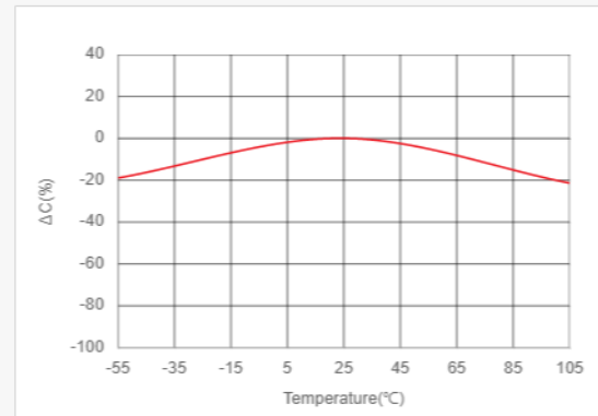
Temperature Characteristics of Capacitance(TCC) LCR meter, 0.12kHz, 0.1Vrms
